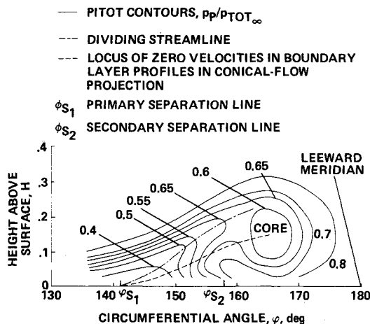
Fig. 7 Computed contours of constant pitot pressure on leeward of cone at M_\infty = 1.8 , \alpha = 11 deg, R_{x_\infty} = 9.8 \times 10^6 .
