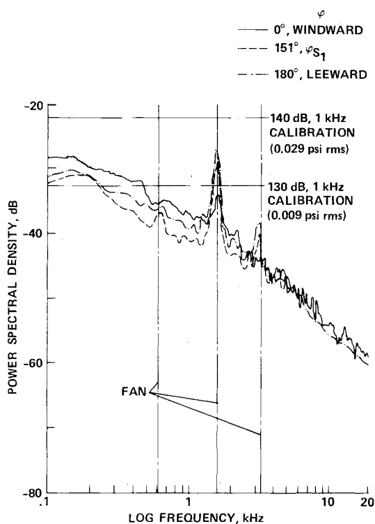
Fig. 10 Wind tunnel power spectral density measurements at windward and leeward rays compared with primary separation line, M_\infty = 1.5 , RN = 2.9 \times 10^6 /ft.
