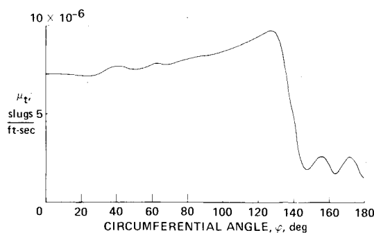
Fig. 12 Circumferential variation of eddy viscosity in numerical computation, M_\infty = 1.5 , \alpha = 11 deg, R_{x_\infty} = 9.8 \times 10^6 /ft.
