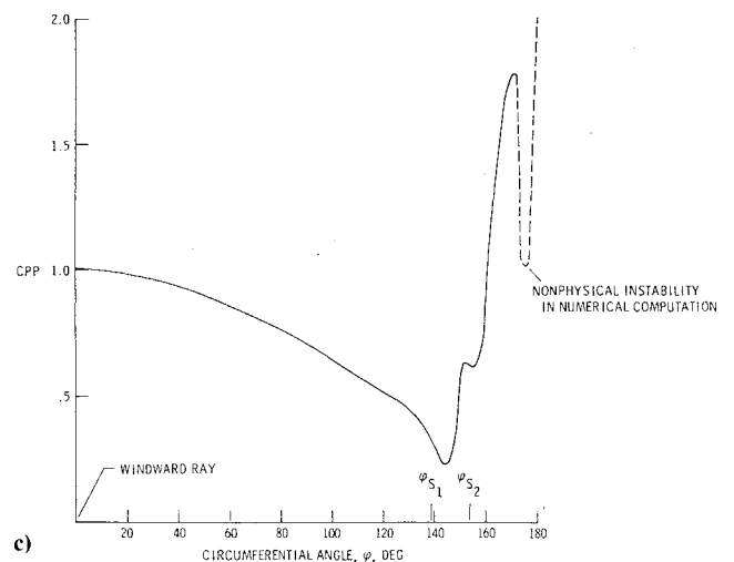
Fig. 6 Flight, wind tunnel, and computed indications of skin friction at M_\infty = 1.8 , \alpha = 11 deg. a) Flight measurements of obstacle block pressures at x = 30 in., RN = 4.2 \times 10^6/\text{ft} . b) Wind tunnel measurements of obstacle block pressures at x = 30 in., RN = 2.6 \times 10^6/\text{ft} . c) Computation of pitot pressure at H = 0.012 above cone surface, R_{x_\infty} = 9.8 \times 10^6 .
